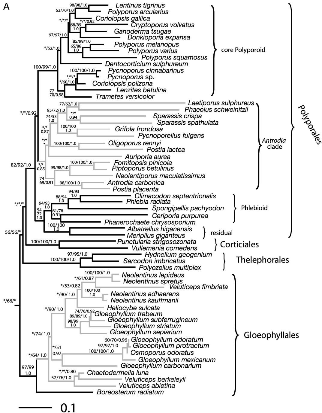
FIG. 2. Phylogenetic relationships of Gloeophyllales inferred with amino acids ( rpb2 , atp6 , tef1 ) and nucleotide (nuc-1su, nuc-ssu, 5.8S rRNA) sequences. Topology from maximum likelihood analysis. Support values along branches from maximum parsimony bootstrap, maximum likelihood bootstrap and Bayesian analyses respectively. Red branches indicate brown-rot lineages. Dashed red branches indicate presumed brown-rot lineages. Blue branch indicates a reversion to white rot in a brown-rot lineage. Branch lengths are drawn proportional to genetic distances (bar = 0.1 average changes per site), except long branches leading to Cantharellus and Agaricomycotina.
