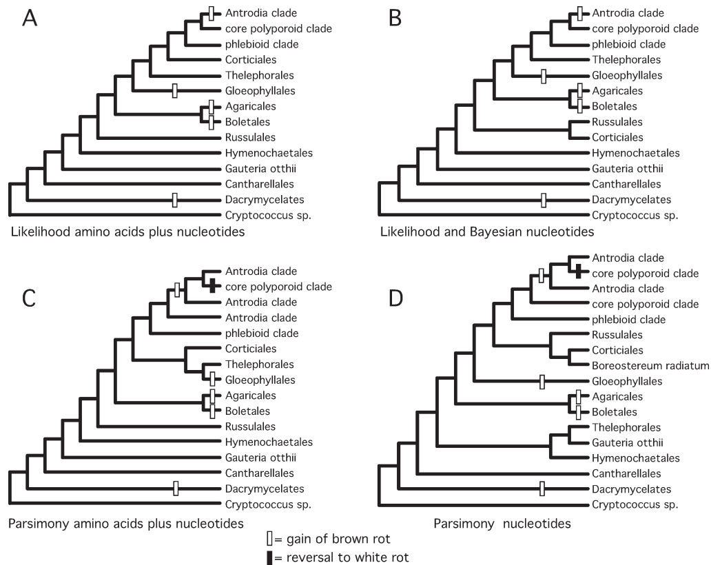
FIG. 3. Simplified phylogenetic topologies and ancestral state reconstructions of the evolution of brown rot. A. Maximum likelihood analysis of amino acids and nucleotides. B. Maximum likelihood and Bayesian analyses of nucleotides. C. Maximum parsimony analyses of amino acids and nucleotides. D. Maximum parsimony analyses of nucleotides. Reconstructions show only gains of brown rot and reversal to white rot in core polyporoid clade (C, D). Reversal to white rot in Grifola frondosa and multiple gains and losses of brown rot in Agaricales and Boletales are not indicated.
