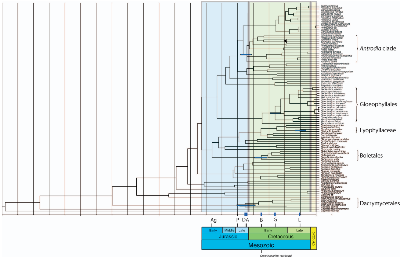
FIG. 4. Chronogram estimated with penalized likelihood analysis implemented in r8s, emphasizing relative ages of brown-rot clades (node height ranges for other clades are not shown). Bars indicate 95% bootstrap node height ranges (node height ranges for other clades are not shown). Triangle indicates putative reversal from brown rot to white rot leading to Grifola frondosa . Mean age of origin of groups indicated with letters above timescale: Ag = Agaricomycetidae, P = Polyporales, D = basal split in Dacrymycetales, A = Antrodia clade, B = Boletales, G = Gloeophyllales, L = Lyophyllaceae.
